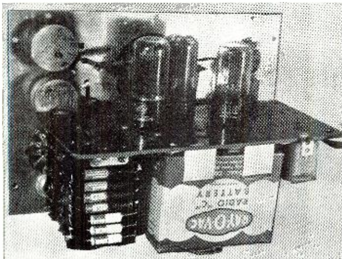
Rear view of the electronic unit.
