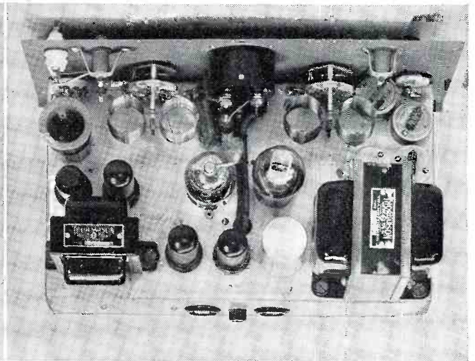
This will give an idea where the parts are placed.
