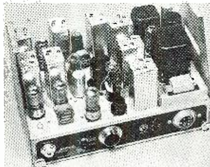
The Motorola FM Police receiver.
