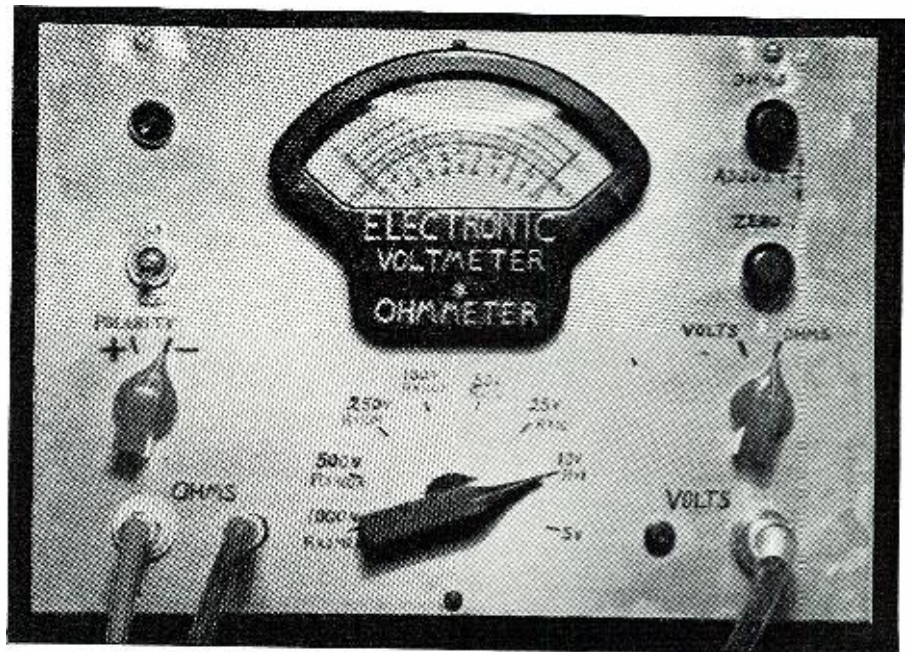
Panel layout of the serviceman's electronic volt-ohmmeter.
