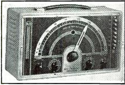
The audio oscillator.
