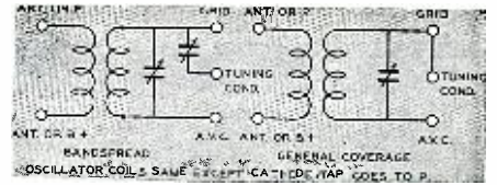
Band-change circuit diagram.
